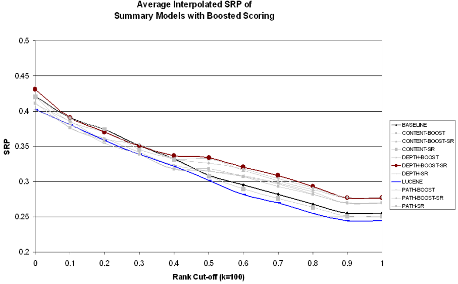
Fig. 5. Structural scoring using boosts and post-processing measured by MASRP
