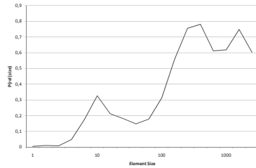
(b) Size prior estimated from the fraction of the number of relevant and retrieved elements
