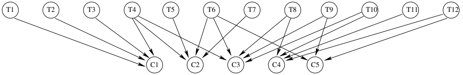
Fig. 2. The OR gate classifier
