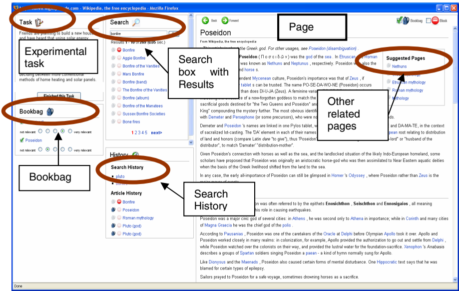
Fig. 1. WikiSearch Interface
