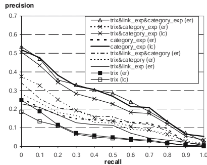
Fig. 4. Recall–precision curves for some of the experimental runs
