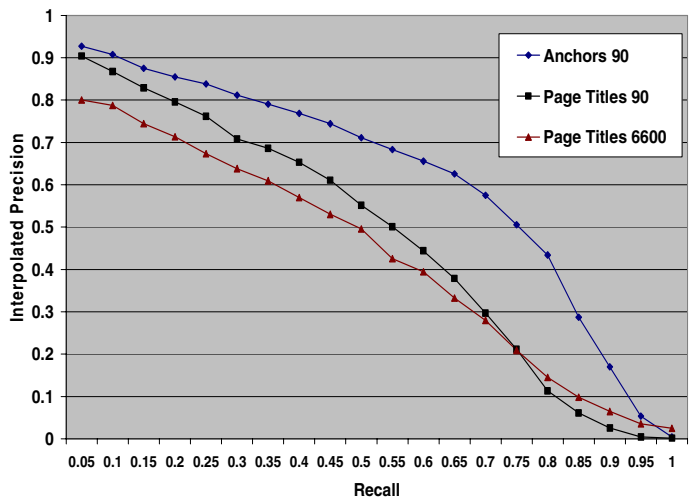
Fig. 4. Link-the-Wiki Outgoing links, interpolated precision vs. Recall
