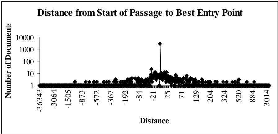
Fig. 5. Distance (in characters) of the best entry points from the start of the first passage. Negative are before the first passage.
